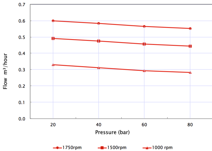
Pump & Power Centre Output Flow
